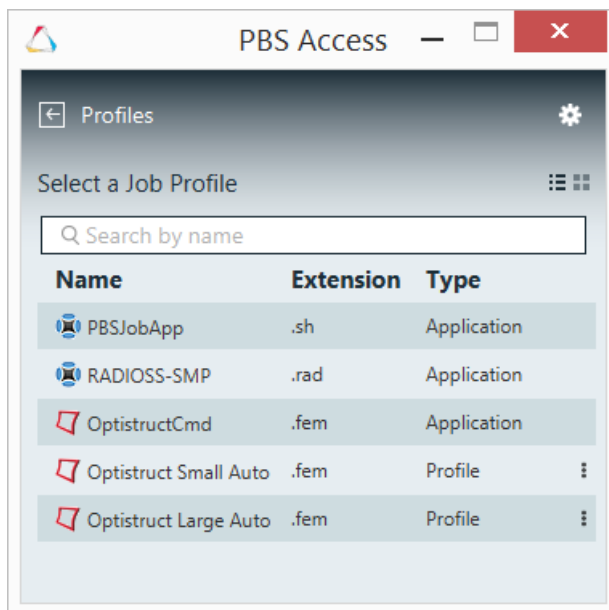
Figure 8: Profile List
