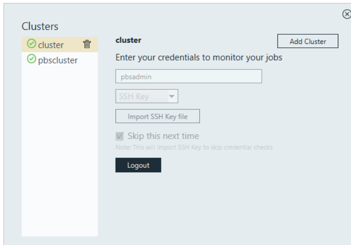
Figure 11: Clusters
