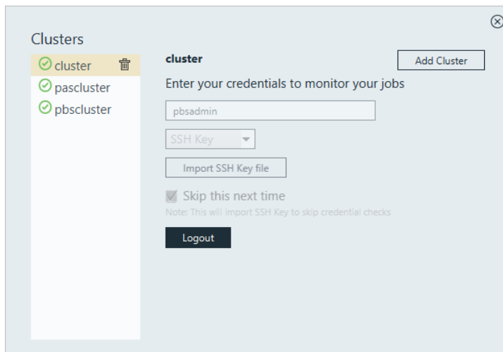
Figure 13: Clusters
